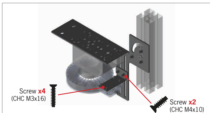
TPL-MOUNT-HPRING-H1
