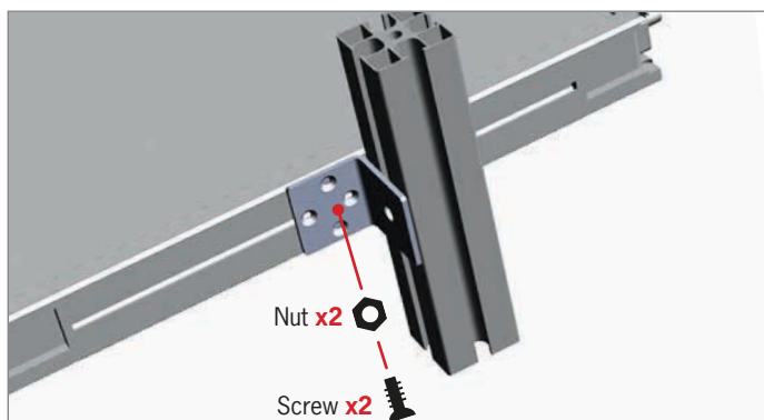
TPL-MOUNT-HPB-SQUARE1
