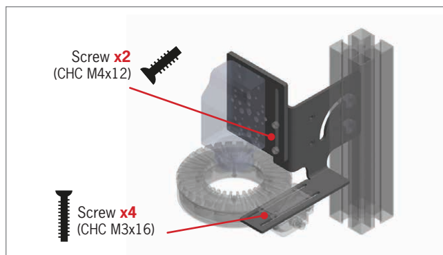
TPL-MOUNT-HPRING-V1
