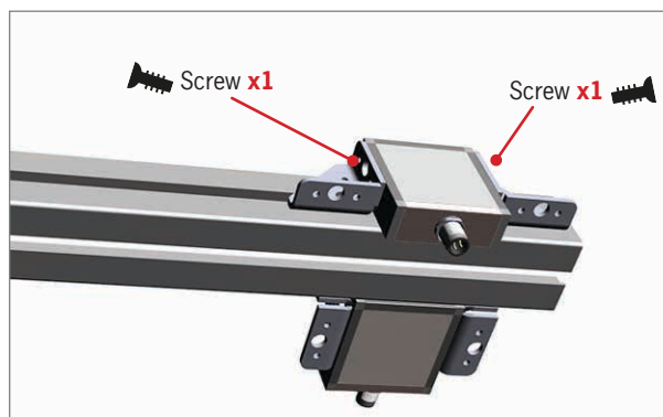
TPL-MOUNT-SBACK-SQUARE1
