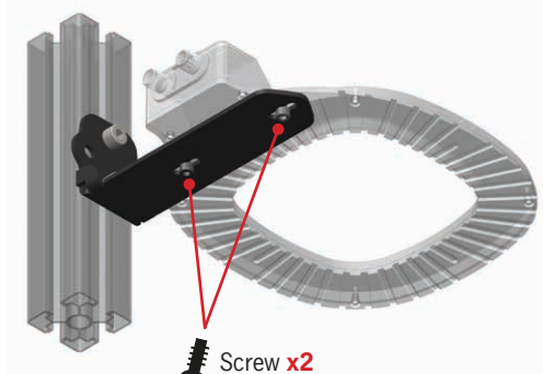
TPL-MOUNT-MR
